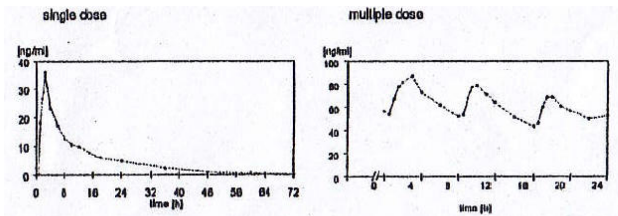
Steady state characteristics of propiverine following multiple-dose administration to 16 healthy volunteers of Mictonom ® 15 mg Coated Tablets (I.I.d for 6 days) :
